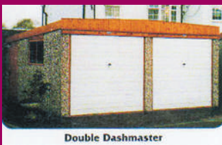
Double Dashmaster
